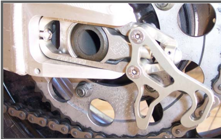
View: KTS-RJ03 chain adjuster with lifter, left side
