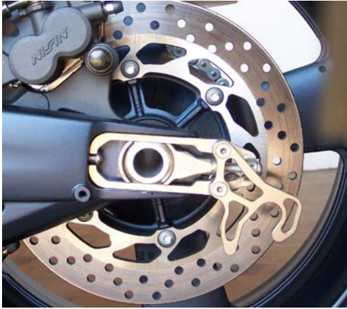
KTS-RP12 titan with lifter
