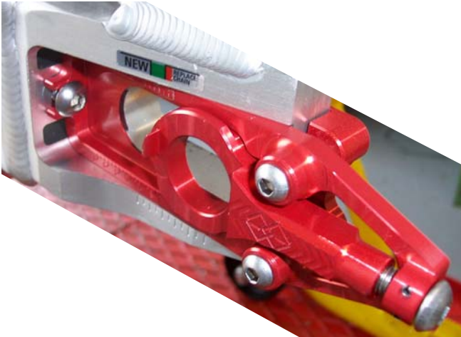
View: KTS-SC57 guidance part with slider and adjusting bolt
